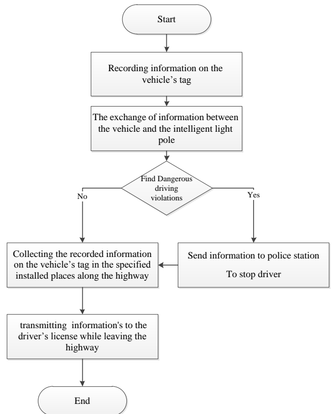
Fig. 6 Flowchart of system steps
